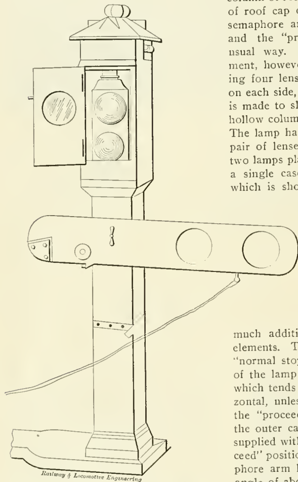
TRAIN ORDER SIGNAL, WITH LAMPS INCASED IN METAL POST.
